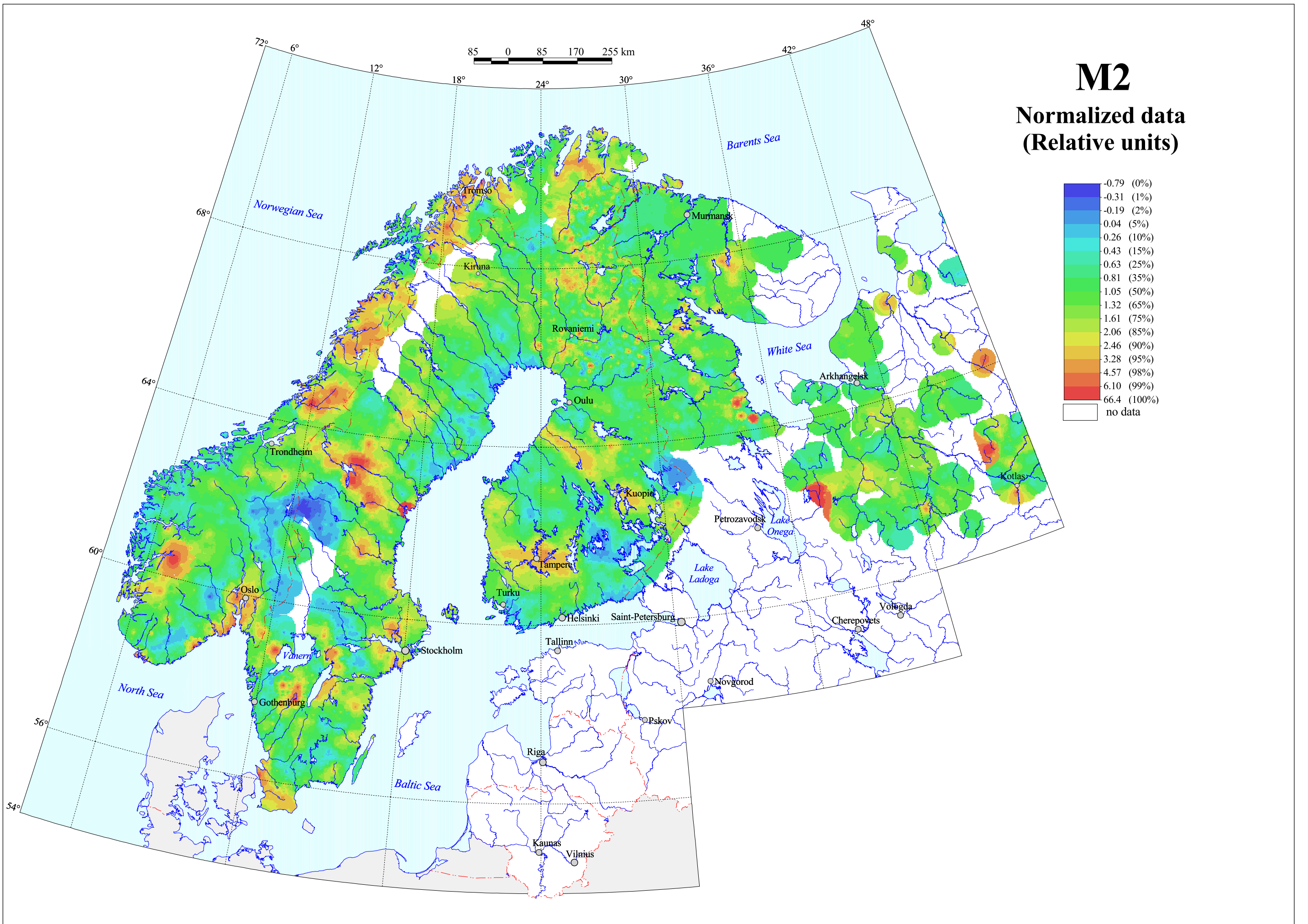
M2 (Fe, Mn) in Till, Grain Size <0.06 mm
